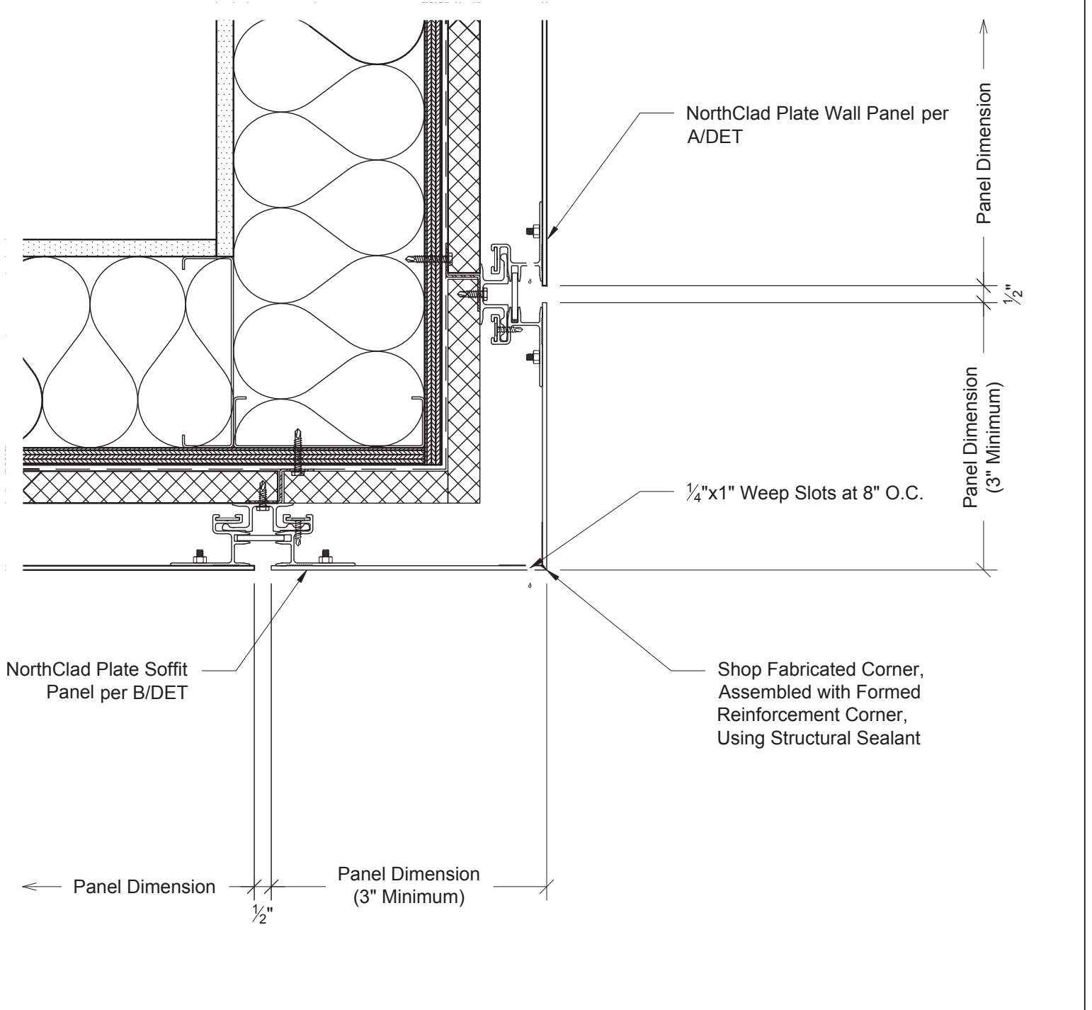
M1 Section - Panels at Fascia to Soffit Transition System: AL-PF with Outboard Insulation
