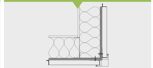
Outside Corner with Trim
