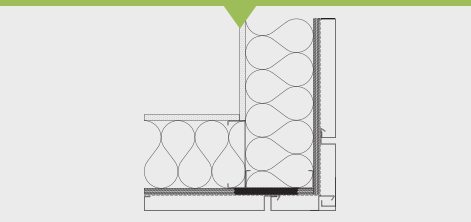
Outside Corner without Trim
