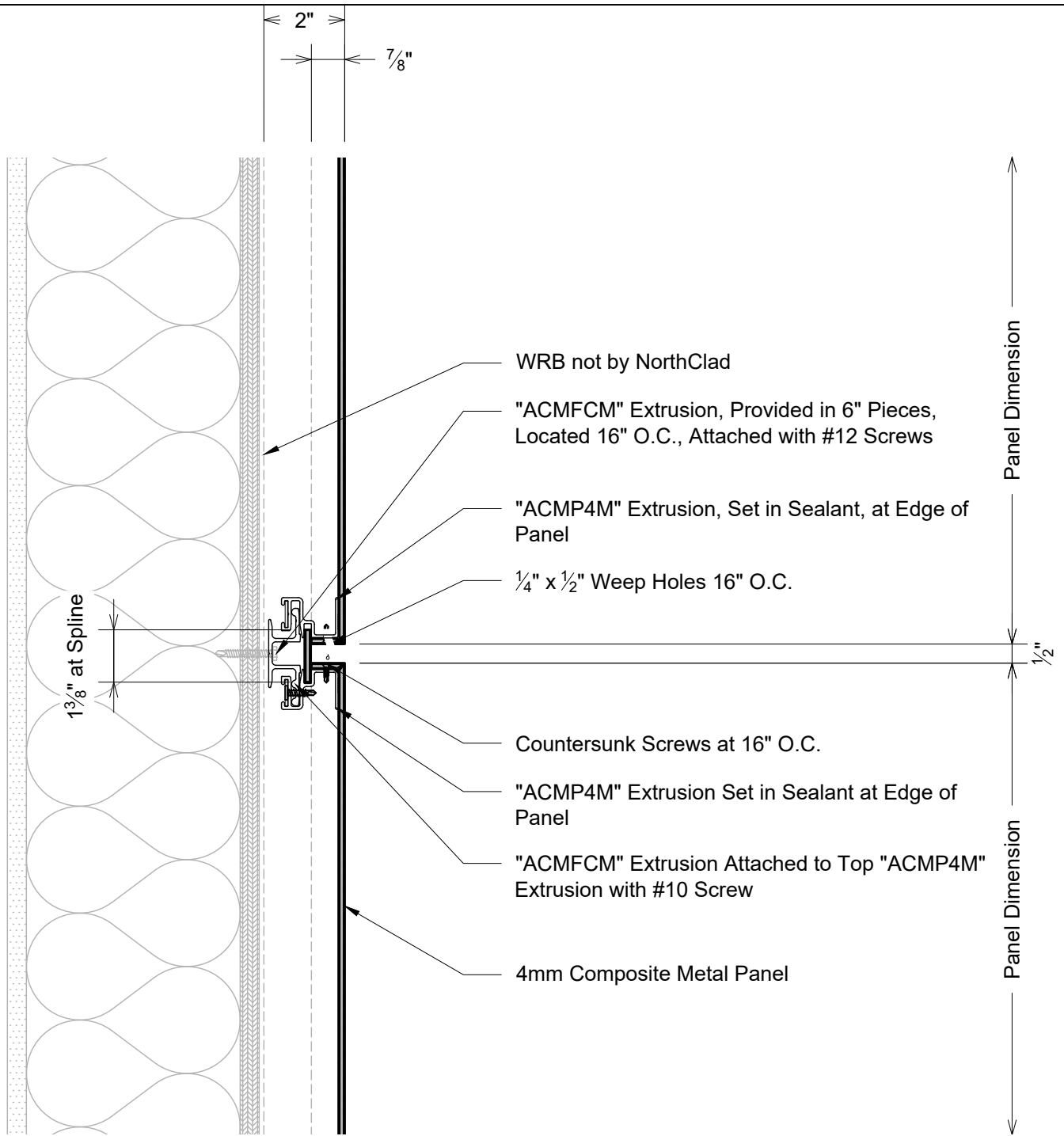
A DET Section - Horizontal Joint
