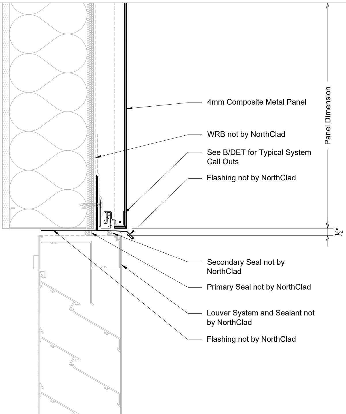
J2 DET Section - Louver Head
