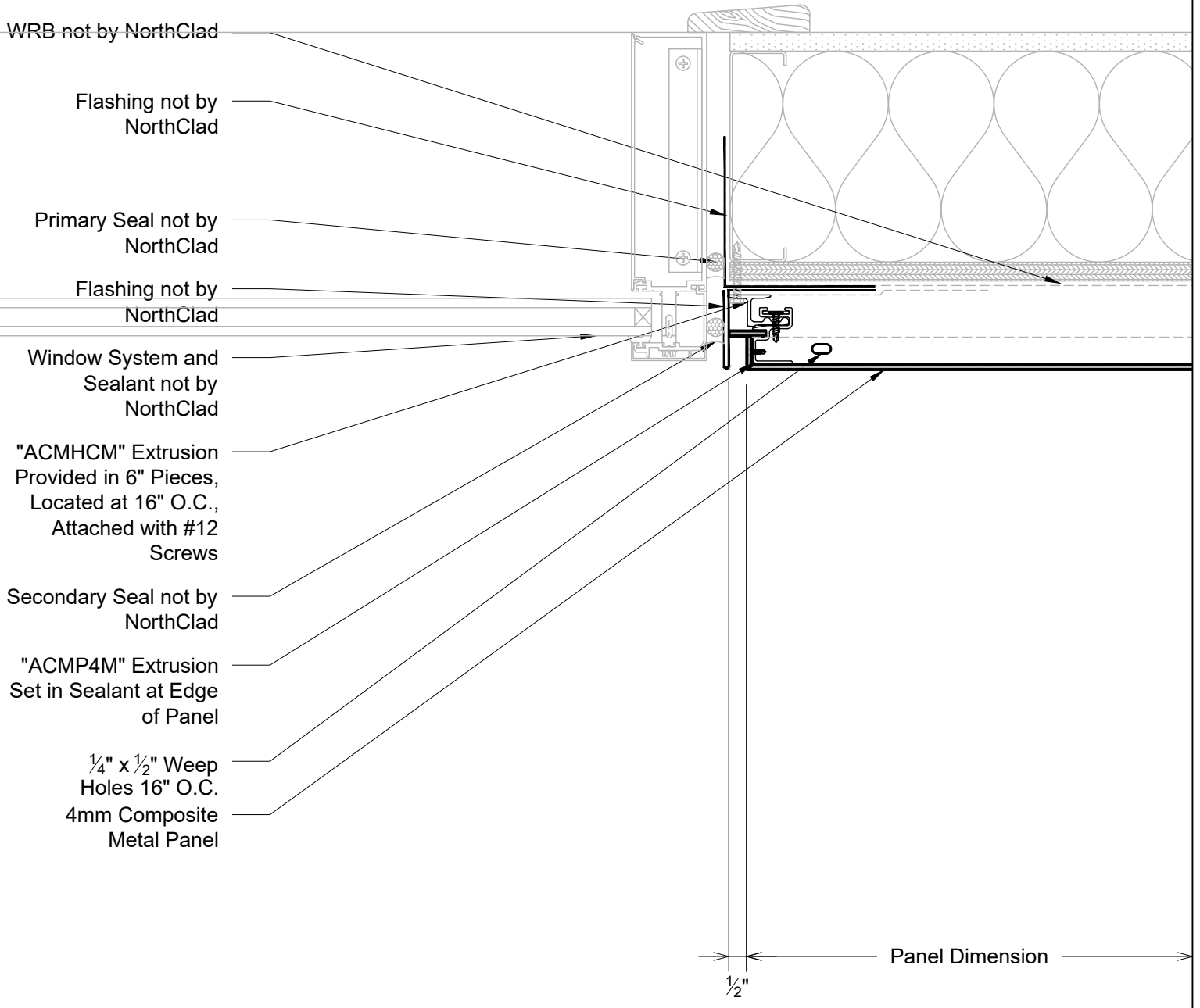
M1 DET Plan - Window at Right Jamb
