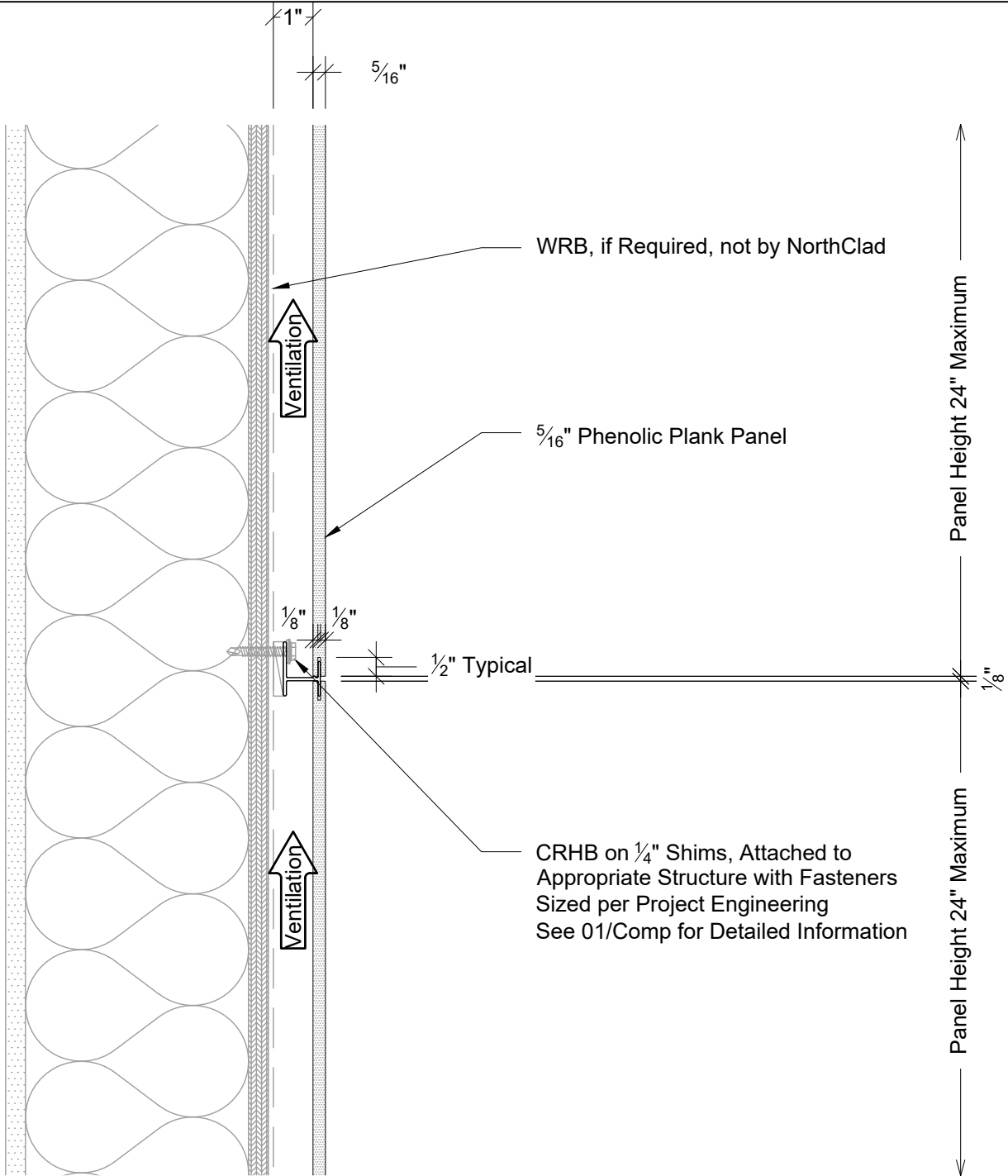
Section - Horizontal Joint
