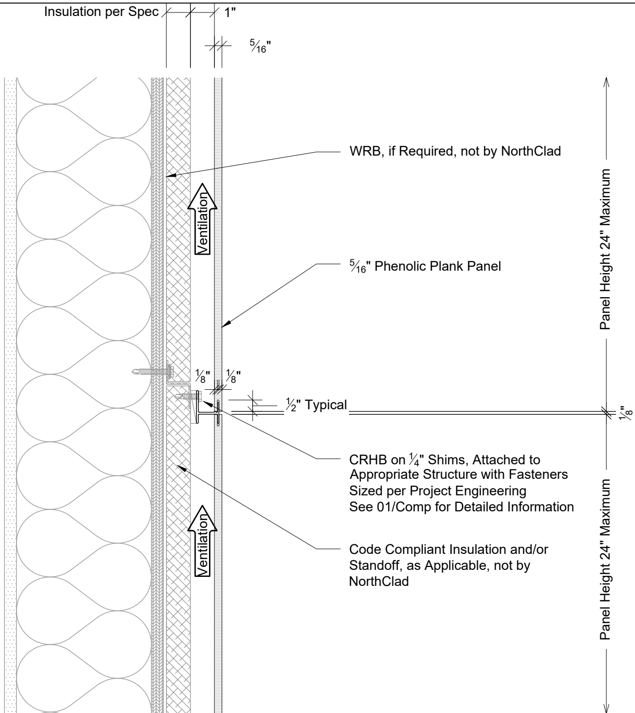
Section - Horizontal Joint
