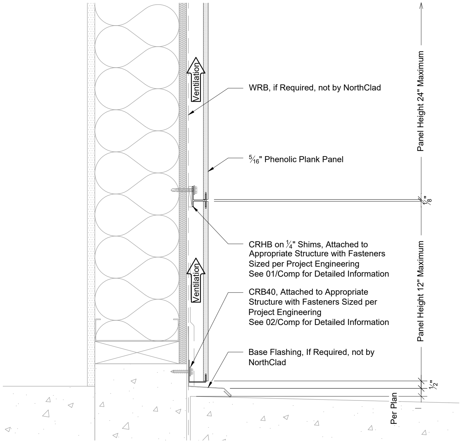
Section - Base of Wall
