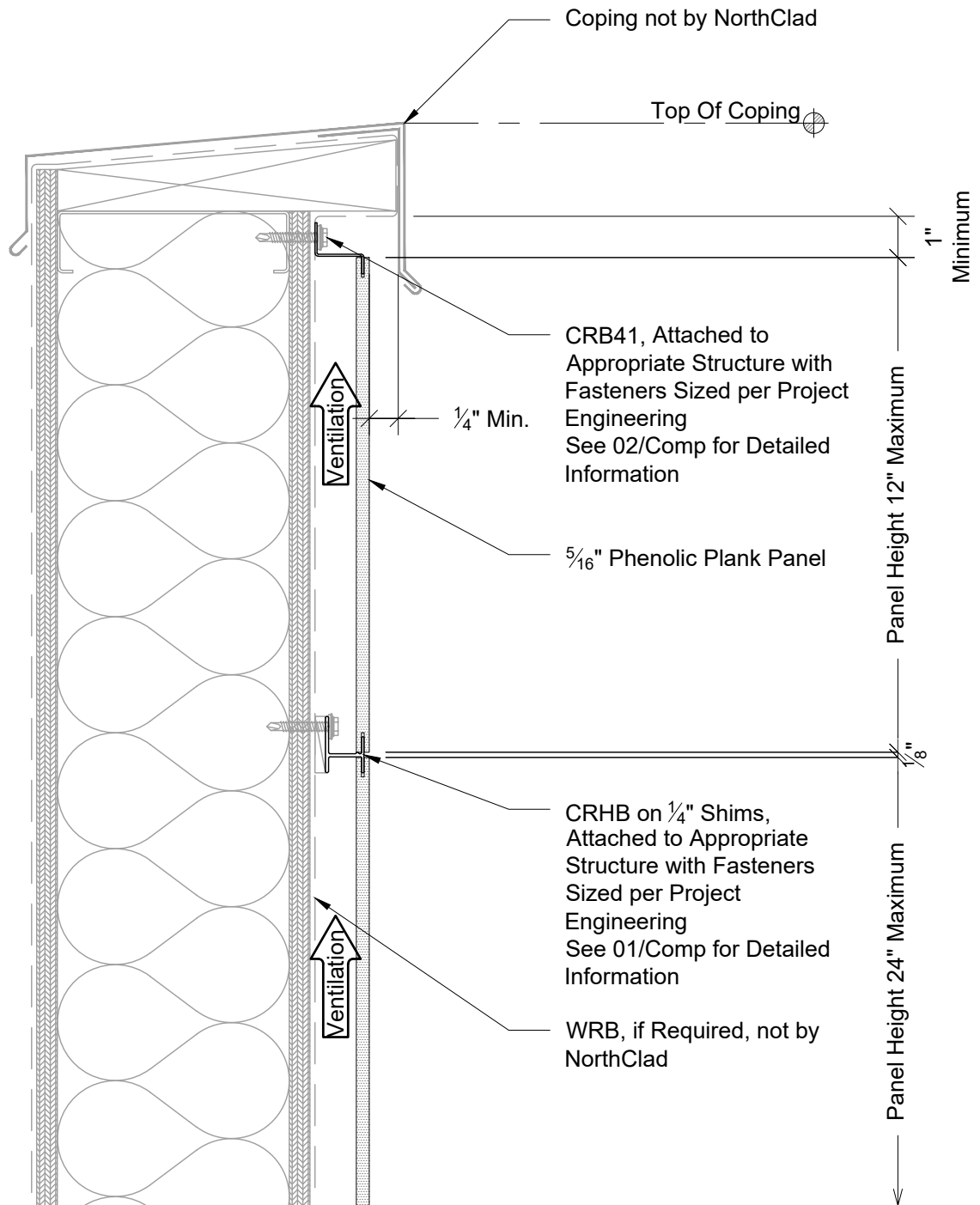
Section - Formed Parapet Coping
