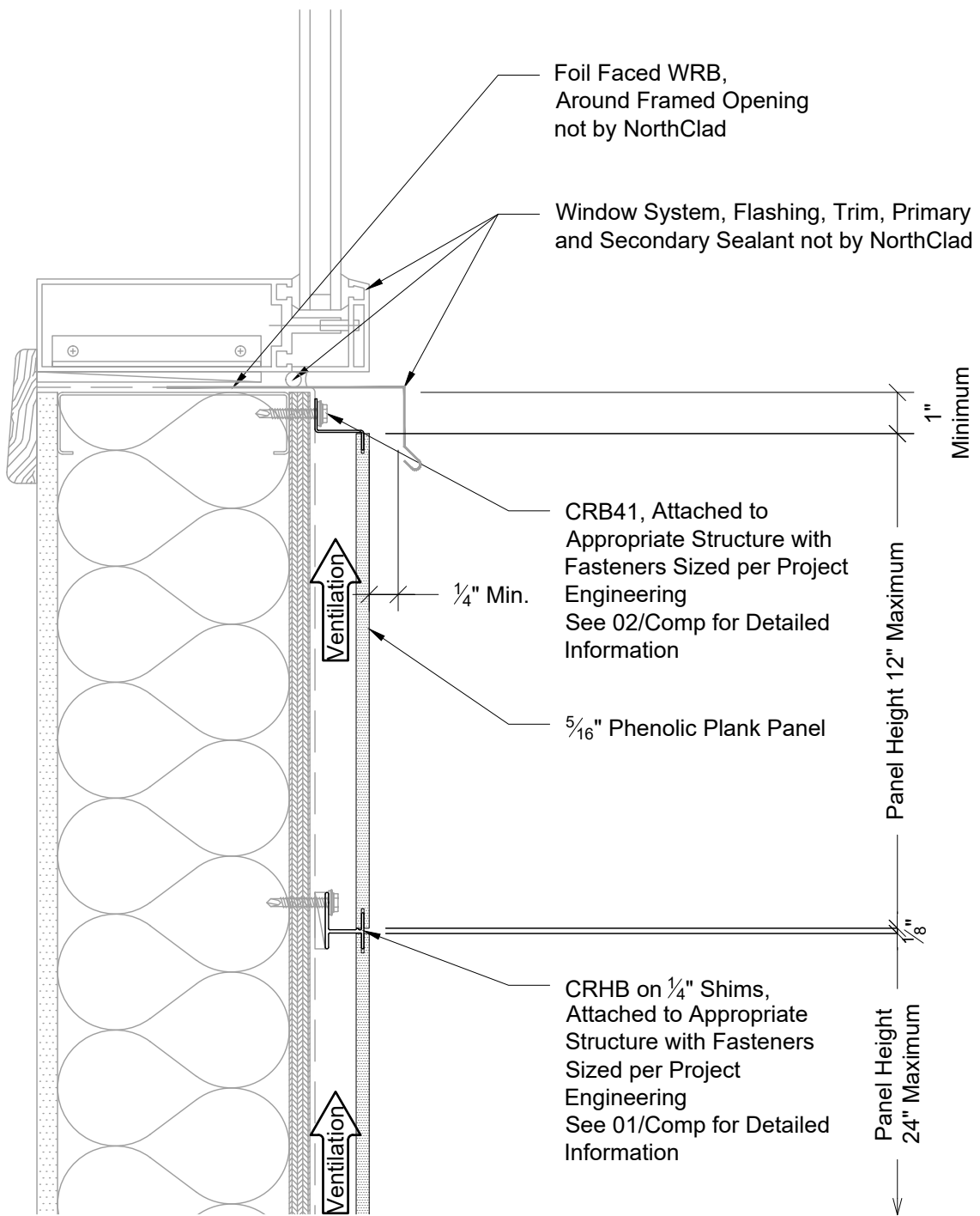
Section - Window Sill
