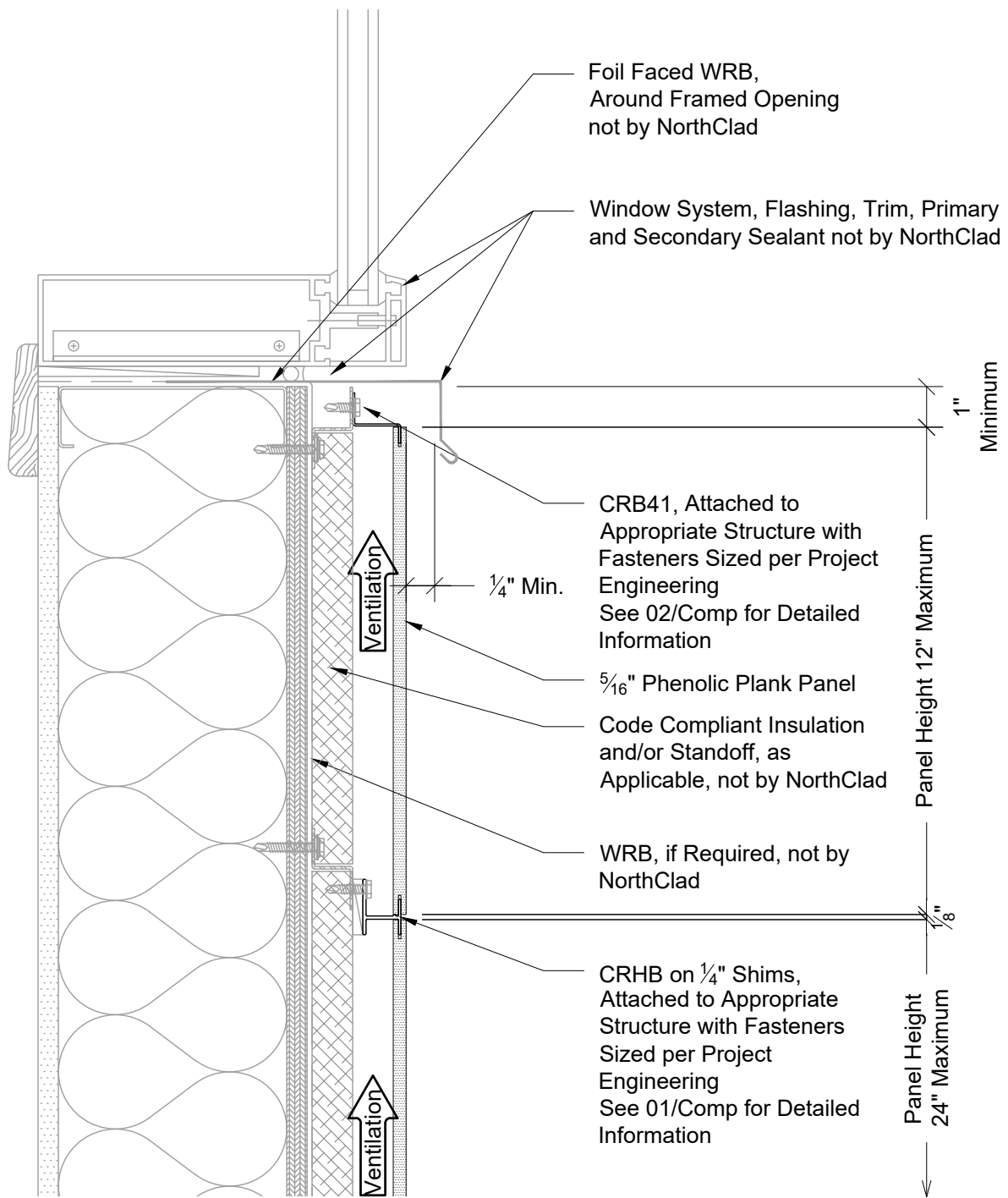
Section - Window Sill
