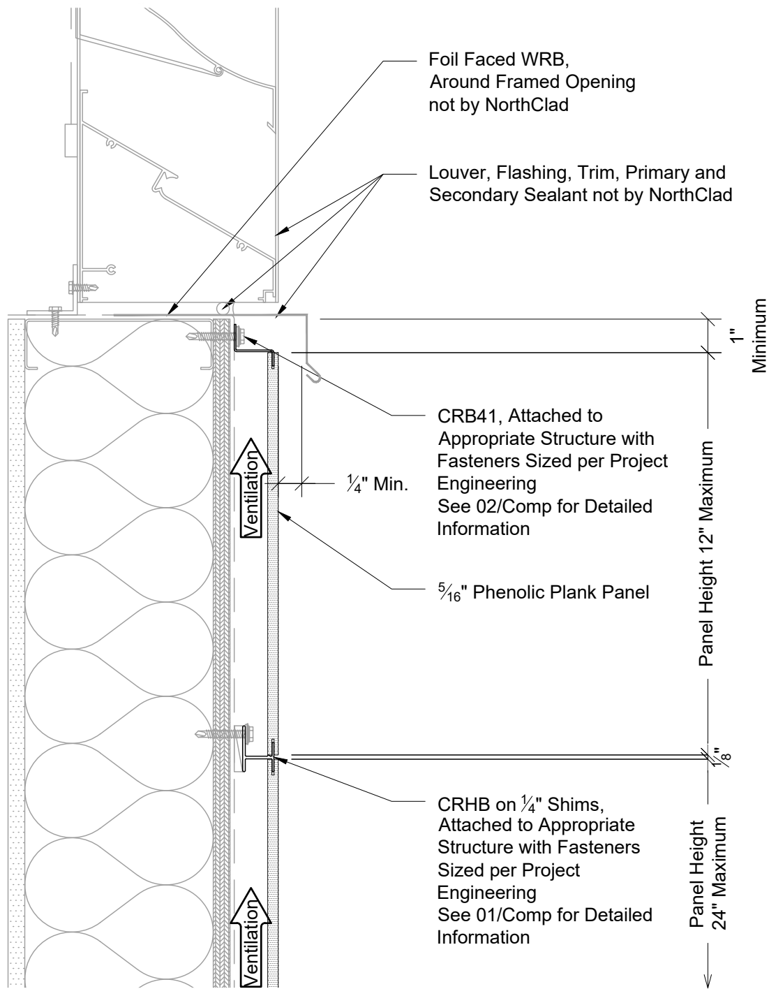
Section - Louver Sill
