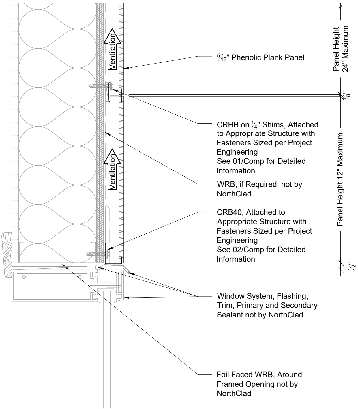
Section - Window Head
