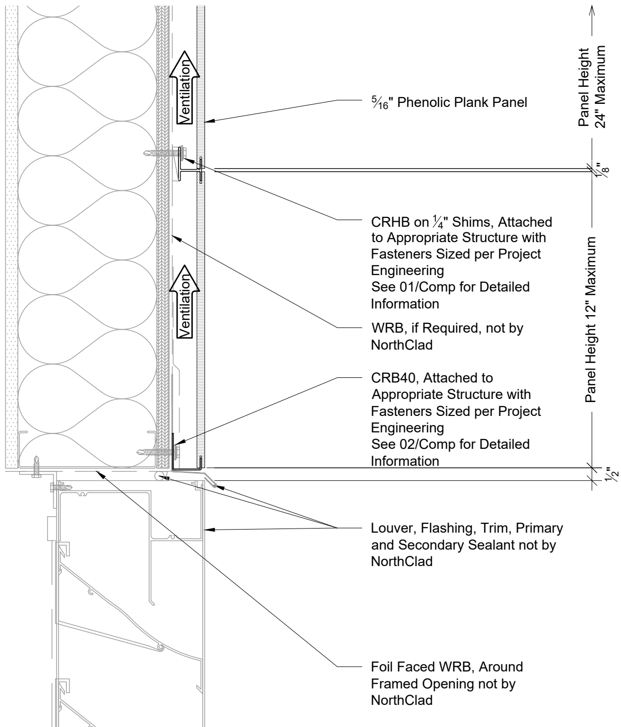
Section - Louver Head
