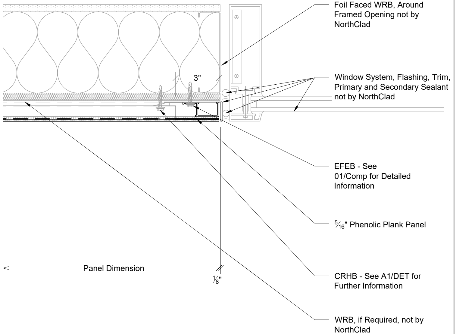
Plan - Window at Left Jamb
