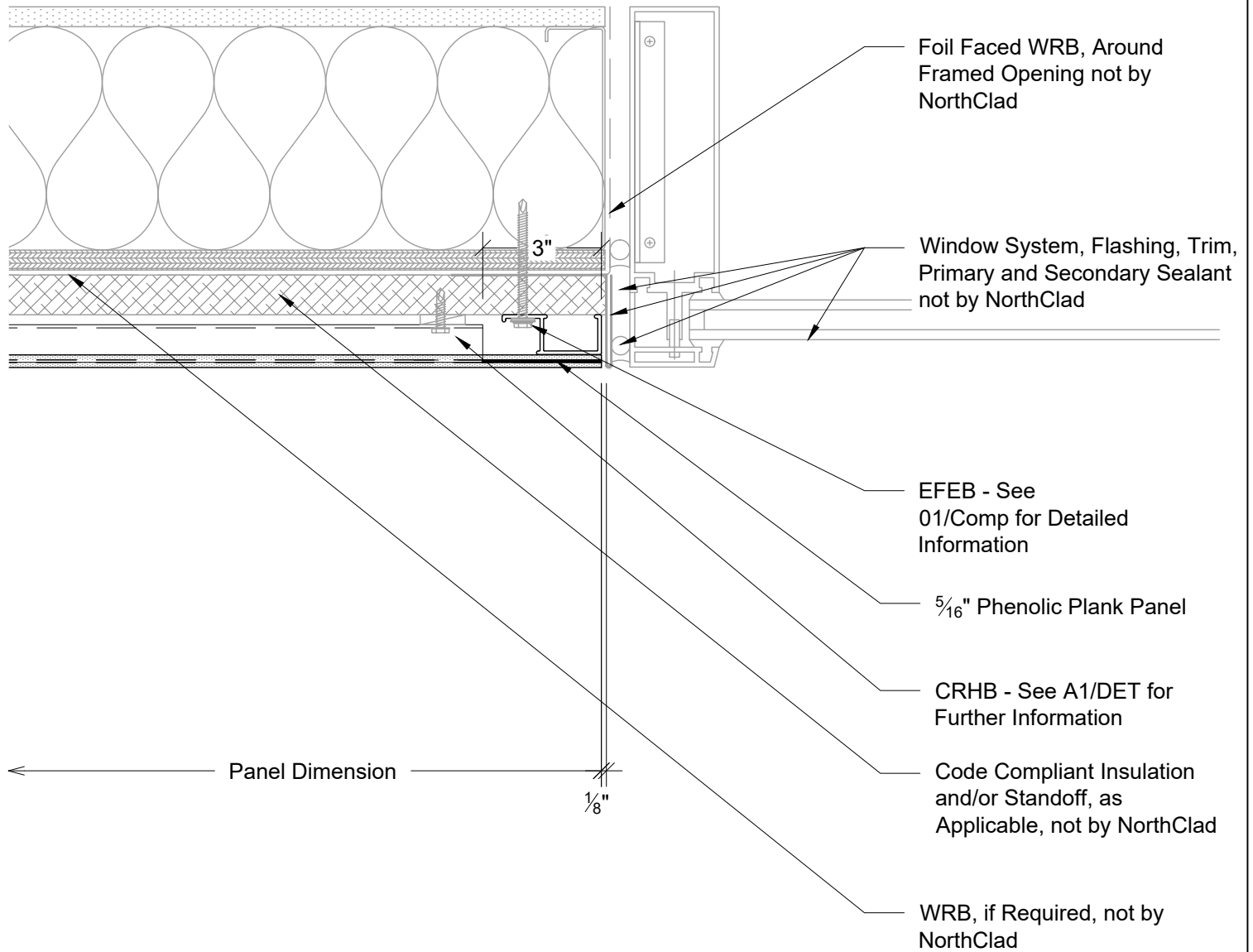
Plan - Window at Left Jamb
