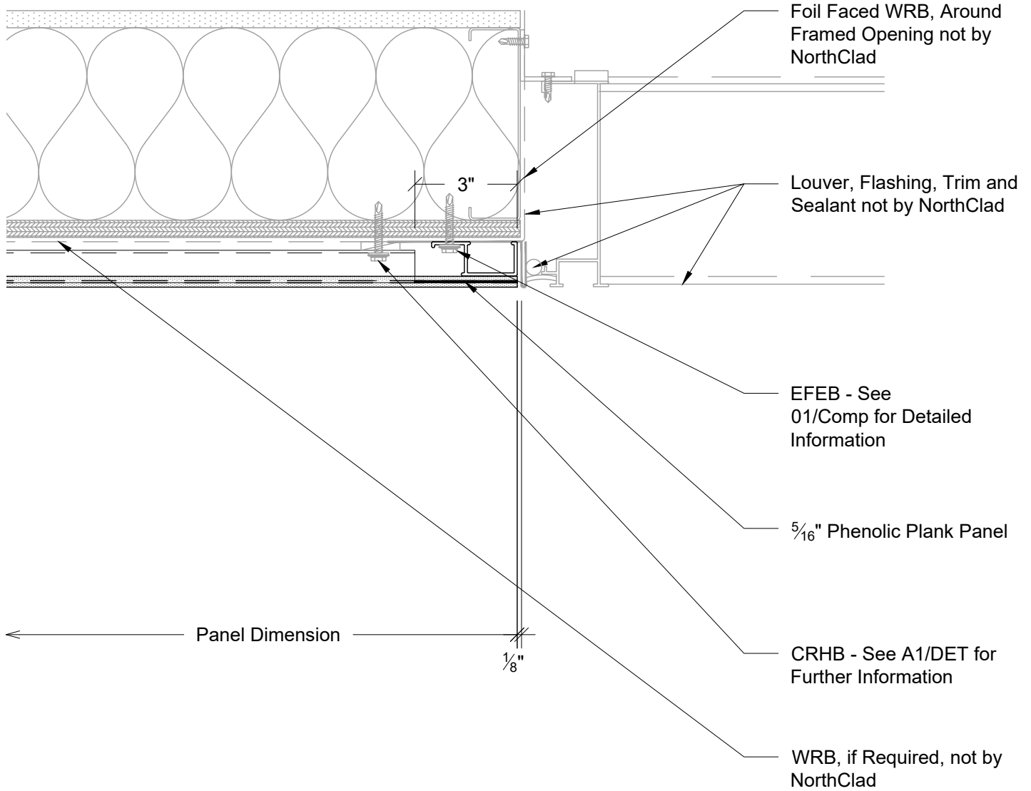
Plan - Louver at Left Jamb
