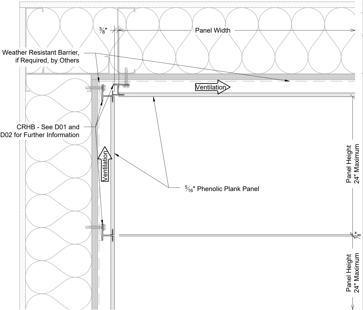
Section - Soffit at Top of Wall
