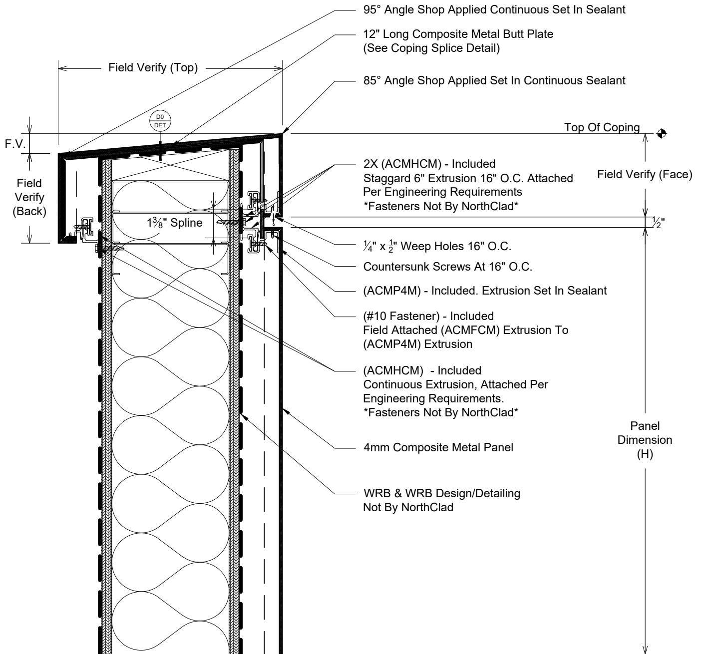
Section - NorthClad ACM - Coping System: NorthClad ACM System
