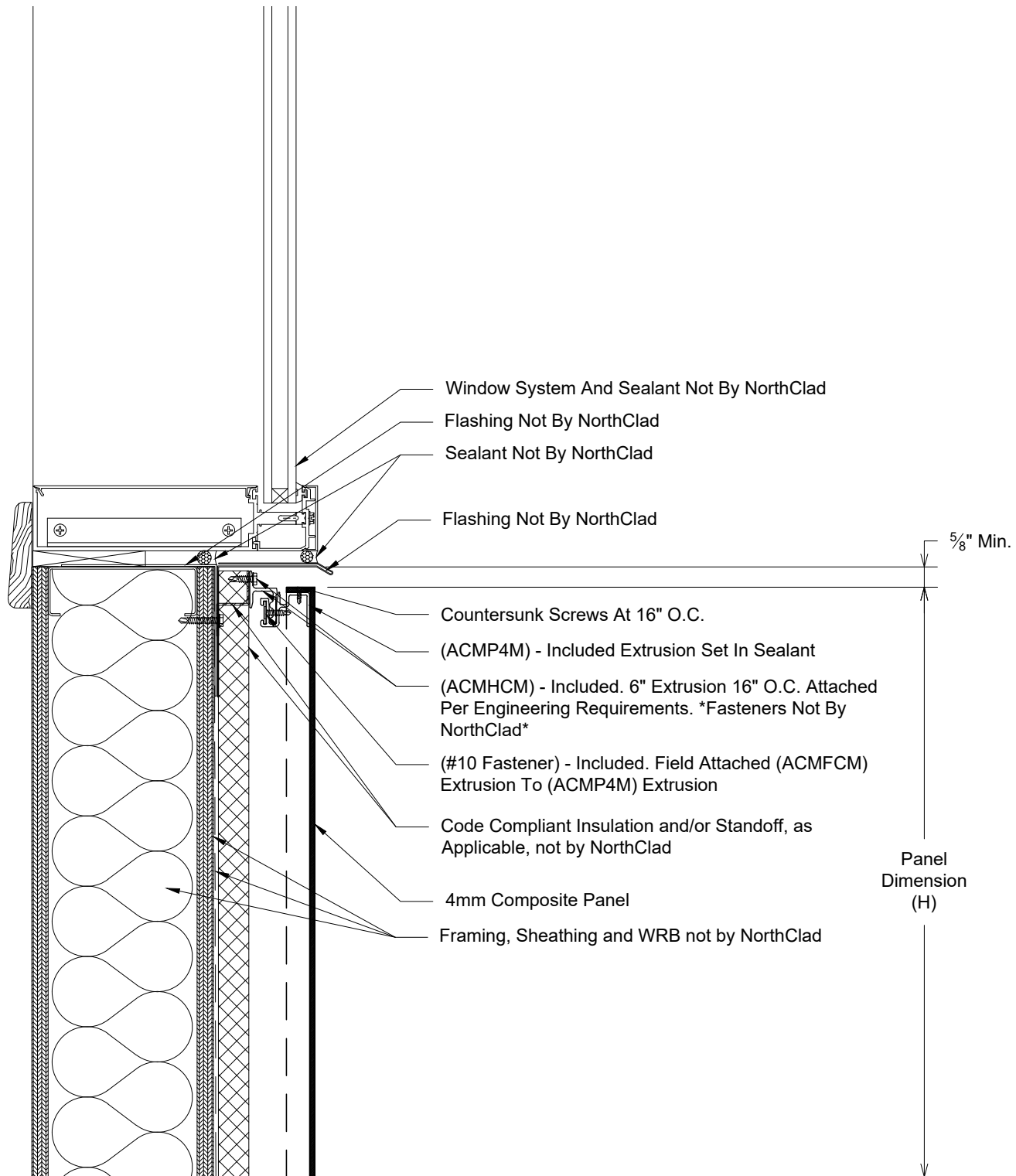
Section - NorthClad ACM - Framed Opening Window Sill System: NorthClad ACM System on Outboard Insulation
