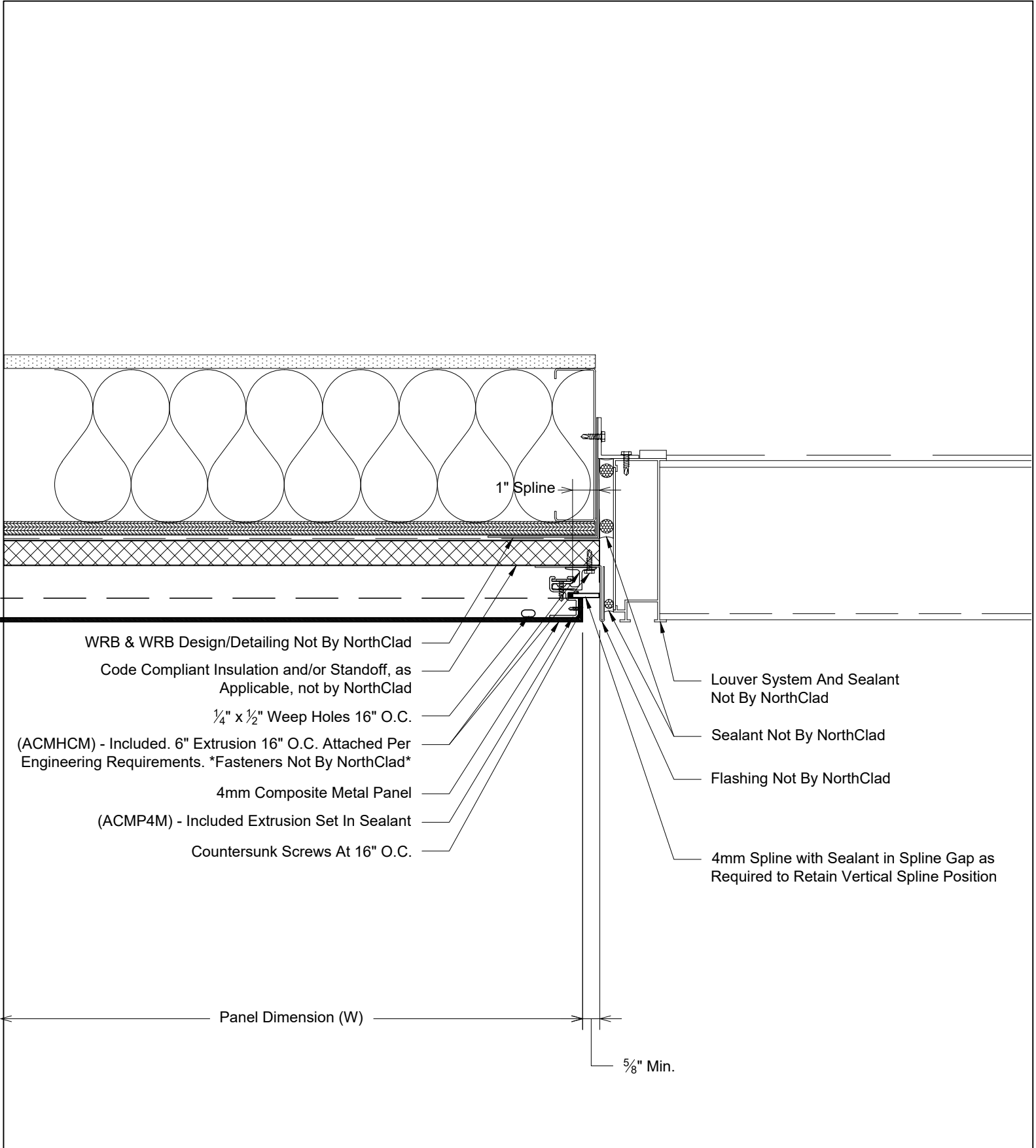
Plan - NorthClad ACM - Framed Opening Louver Jamb System: NorthClad ACM System on Outboard Insulation
