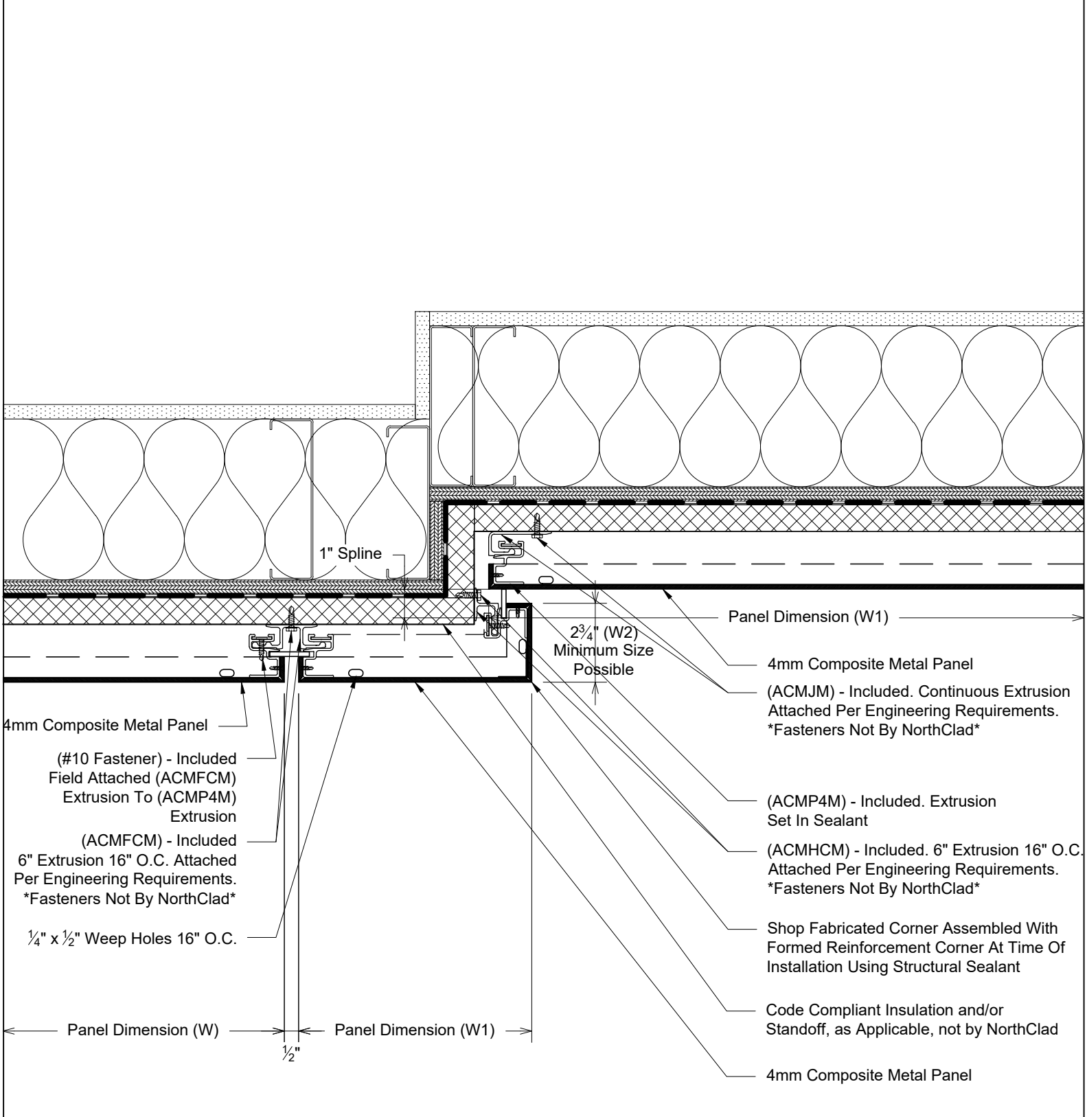
Plan - NorthClad ACM - Minimum Outside Corner System: NorthClad ACM System on Outboard Insulation
