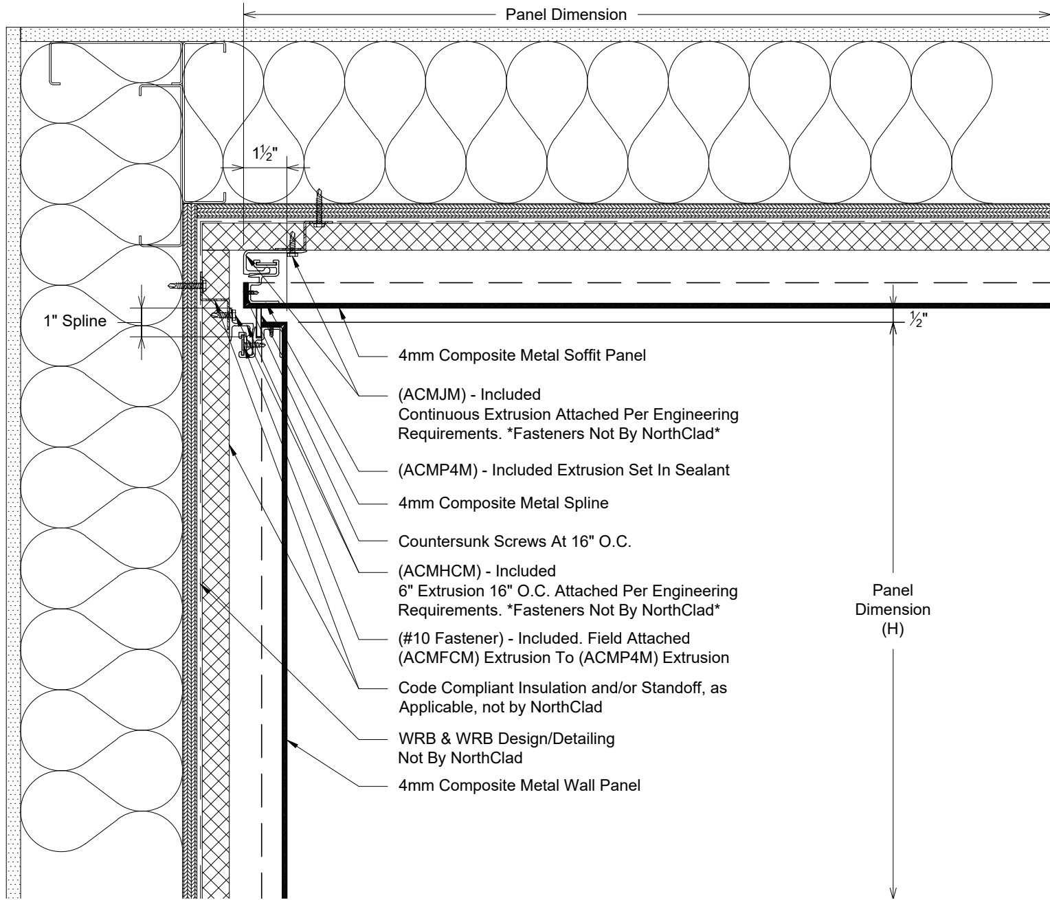
Section - NorthClad ACM - Soffit to Wall Inside Corner System: NorthClad ACM System on Outboard Insulation
