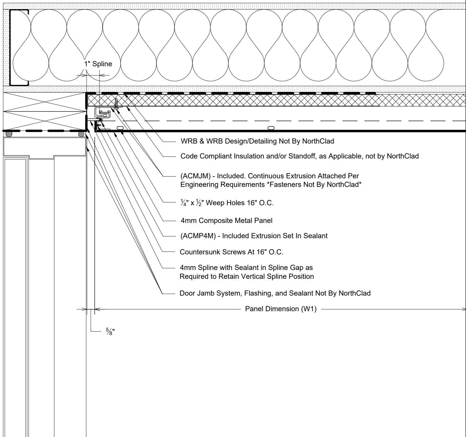
Plan - NorthClad ACM - Inside Corner to Jamb System: NorthClad ACM System on Outboard Insulation
