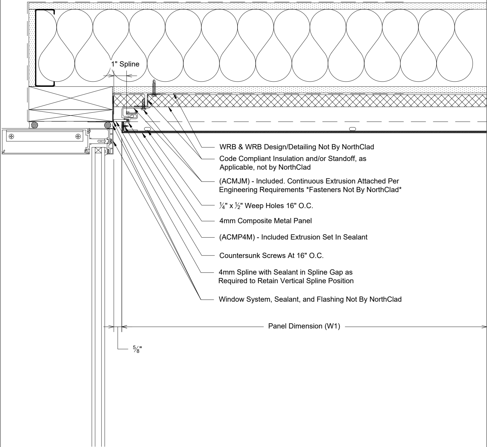
Section - NorthClad ACM - Soffit to Window Header System: NorthClad ACM System on Outboard Insulation
