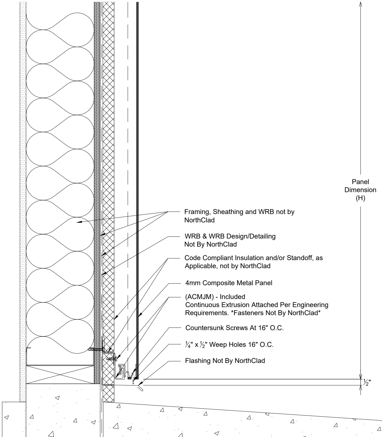
Section - NorthClad ACM - Base of Wall System: NorthClad ACM System on Outboard Insulation
