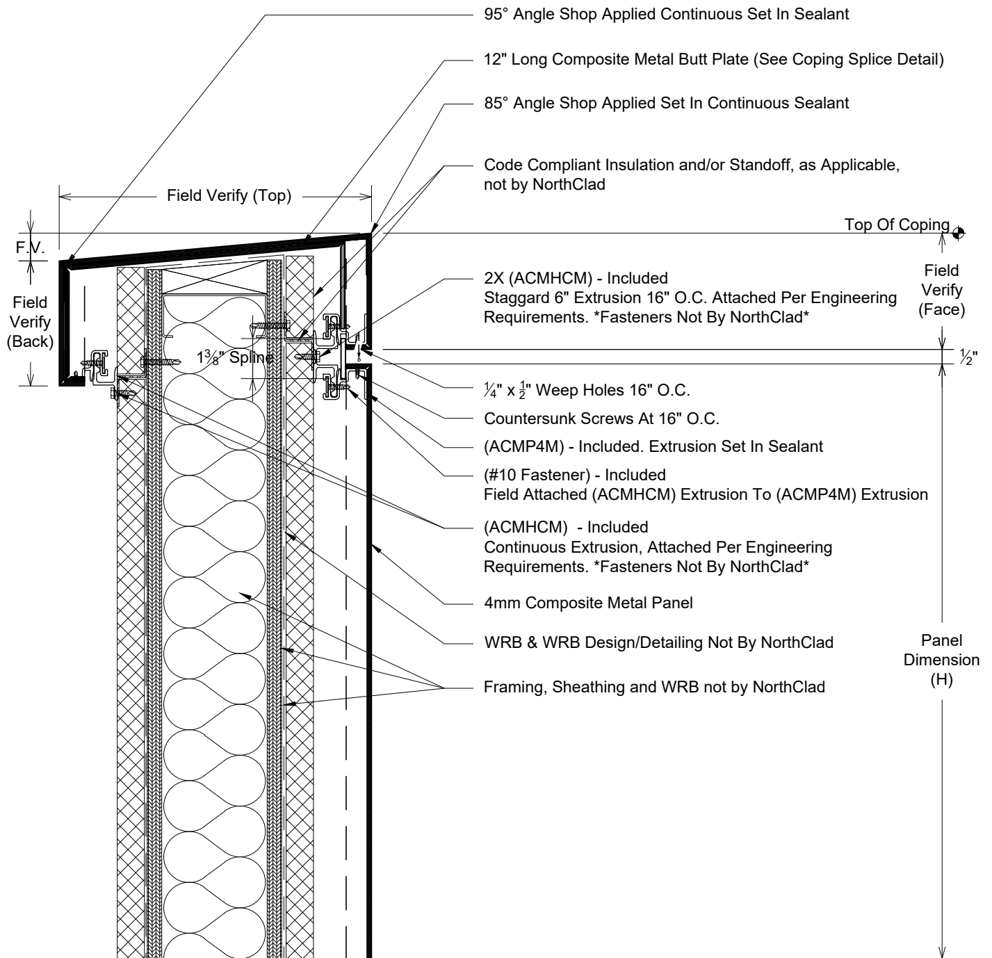
Section - NorthClad ACM - Coping System: NorthClad ACM System on Outboard Insulation
