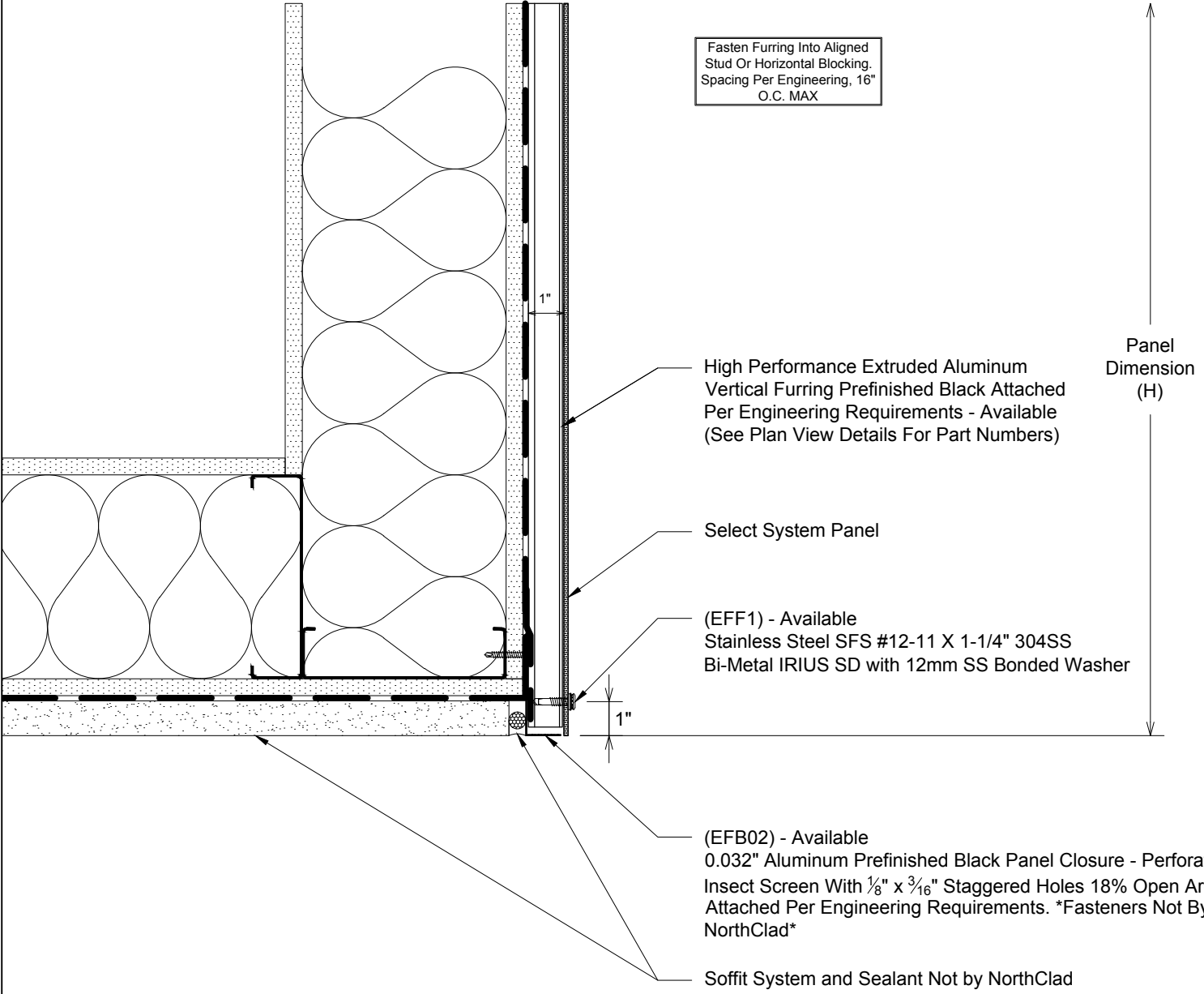
Section - NorthClad EF - Fascia to Soffit by Others System: NorthClad EF System
