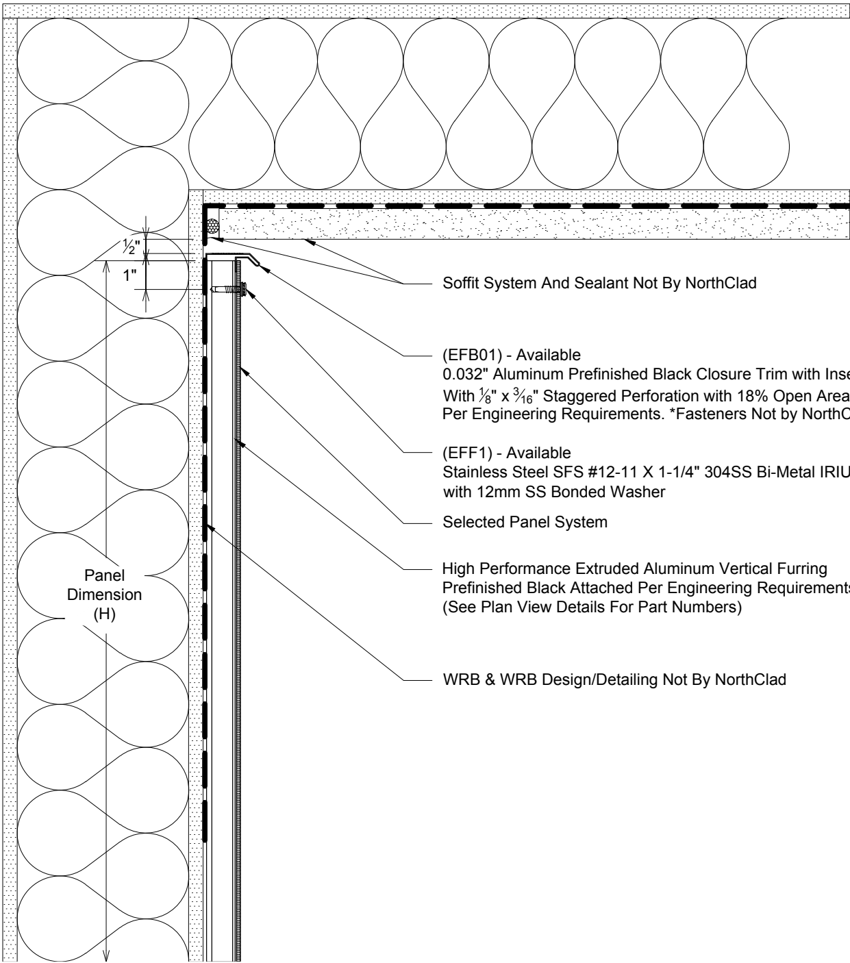
Section - NorthClad EF - Wall to Soffit by Others System: NorthClad EF System
