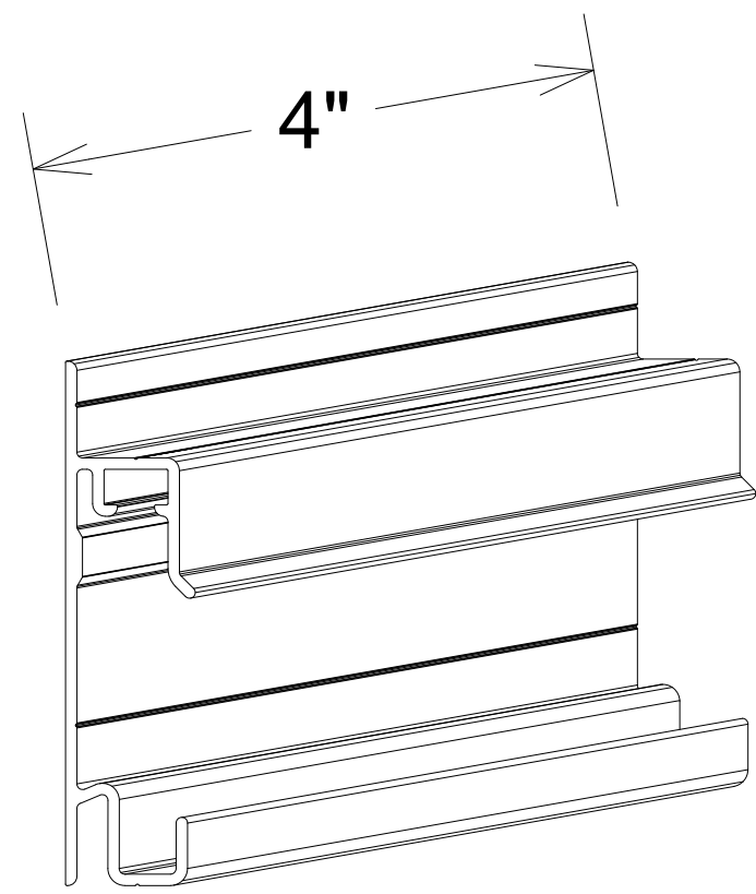
CFCU: Panel Clip Extrusion without Holes
