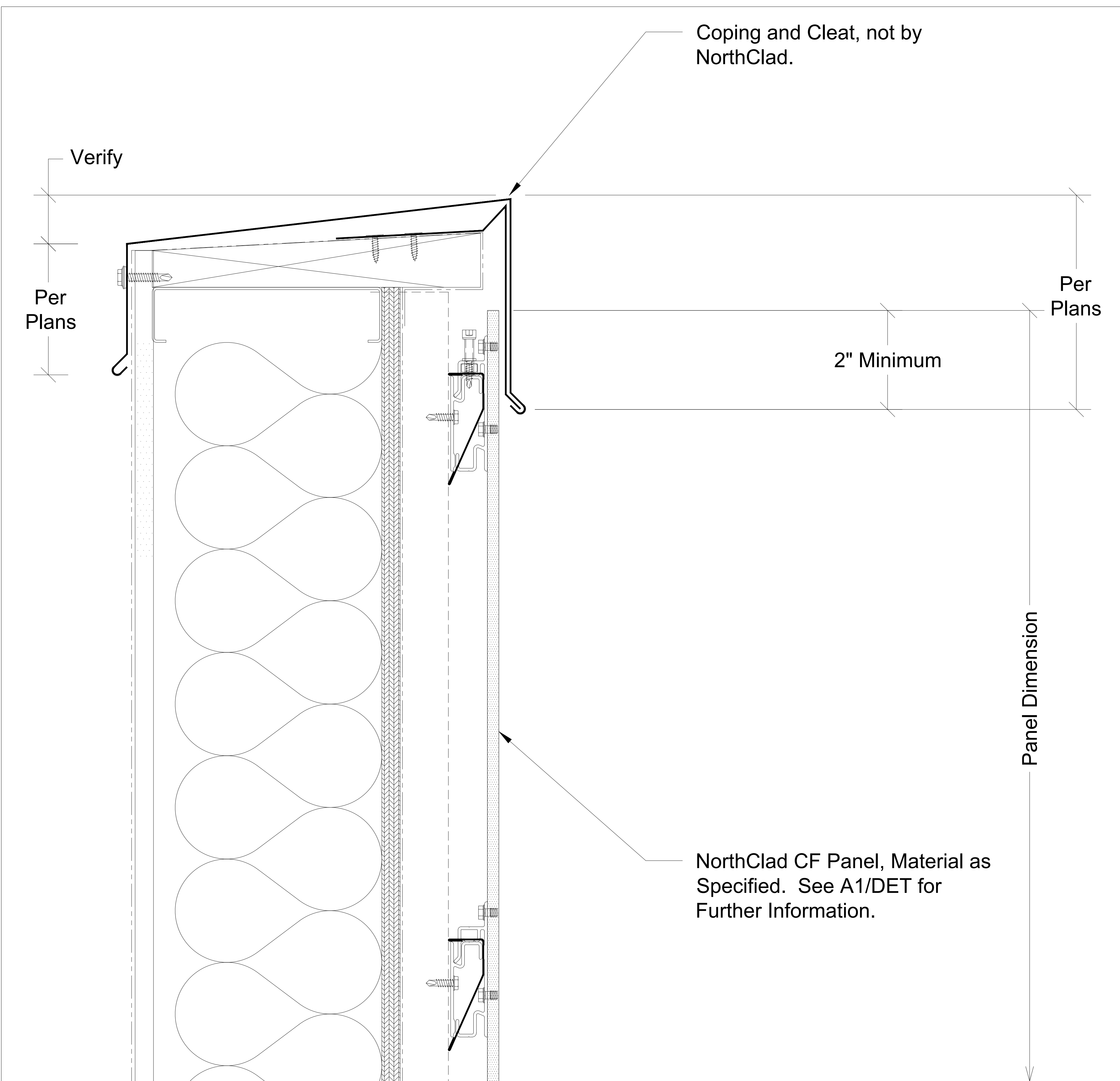
Section - Formed Parapet Coping
