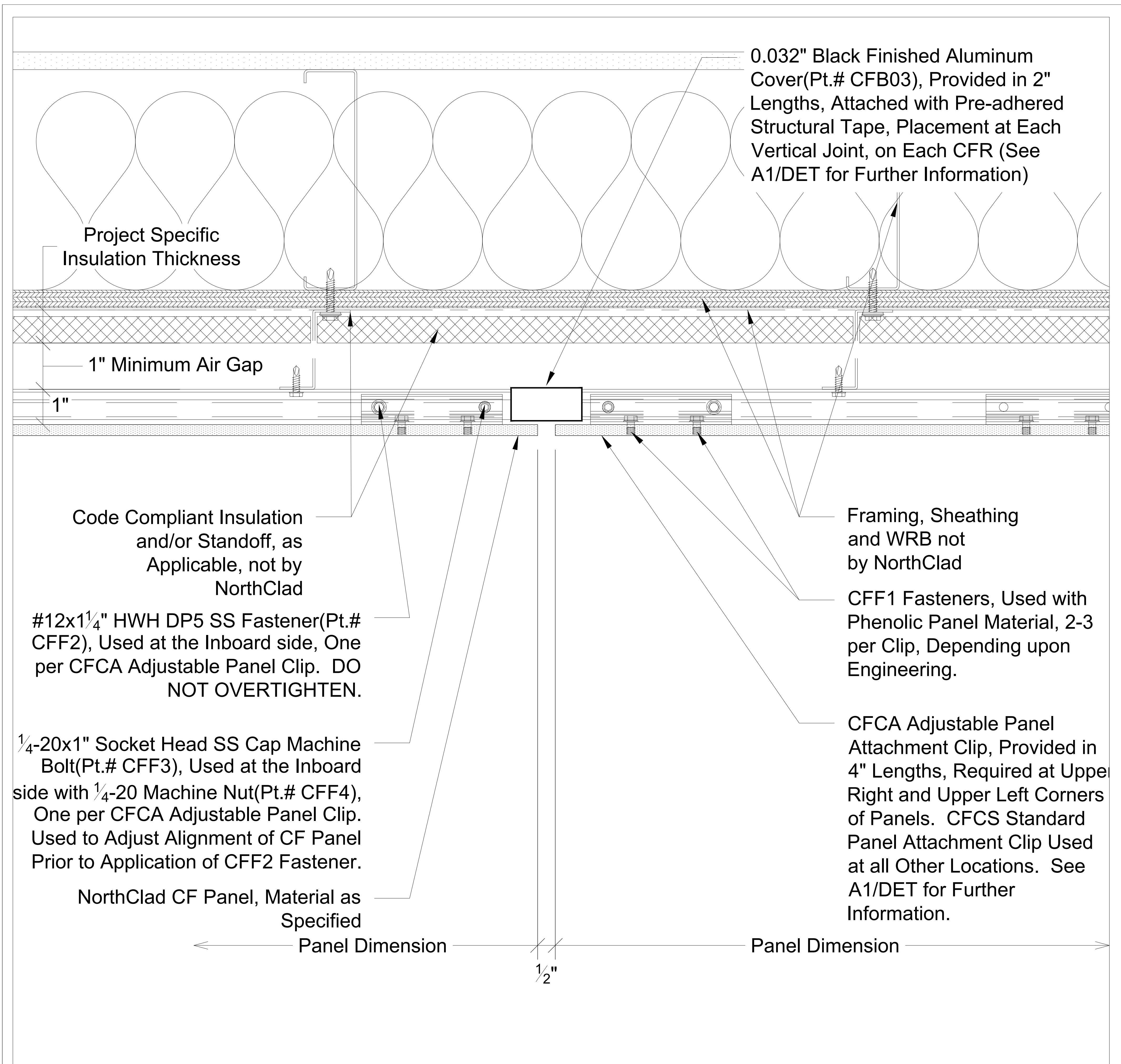
B1 Plan - Vertical Joint
