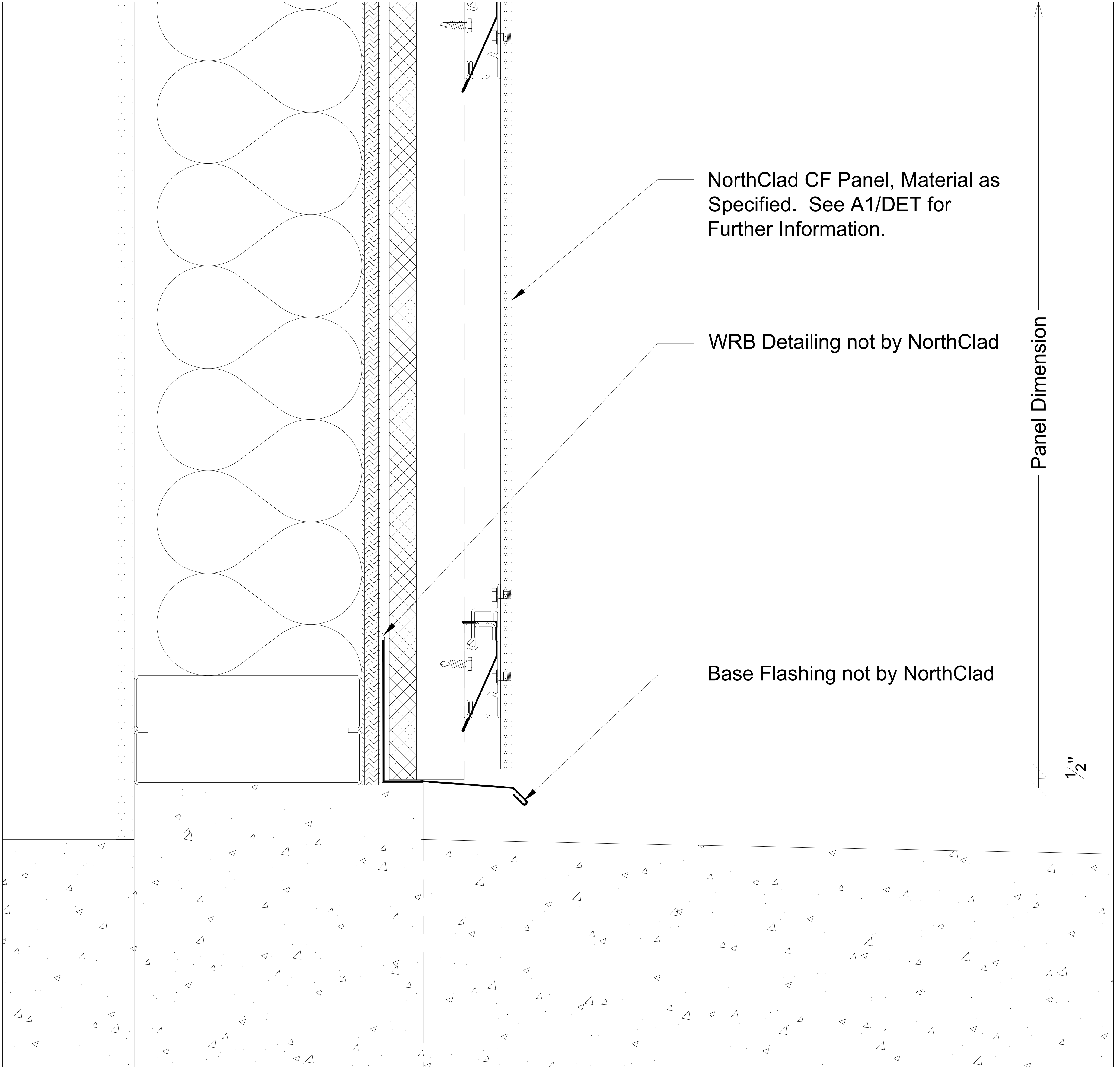
C1 Section - Base of Wall
