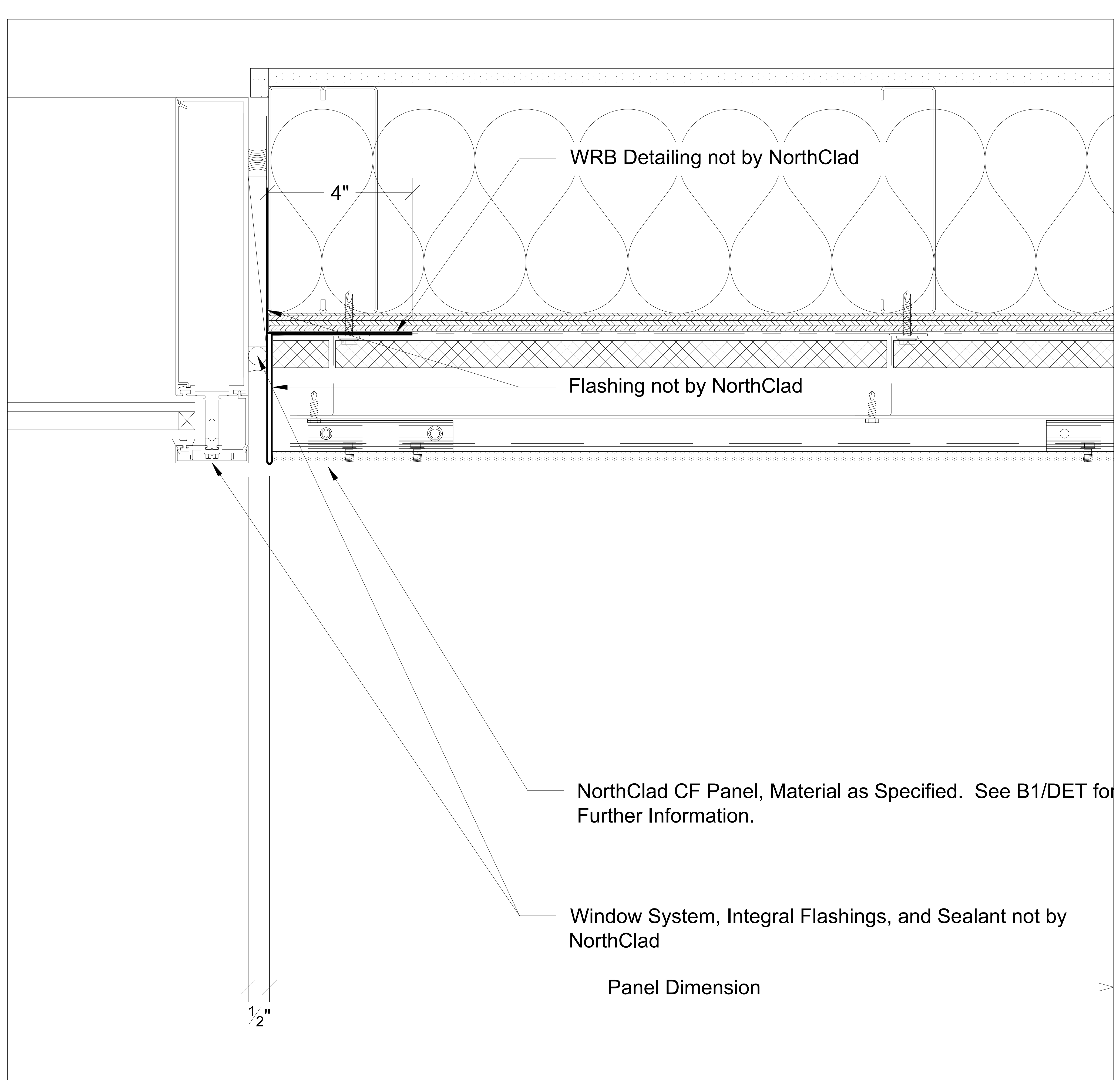
M1 Plan - Window at Right Jamb
