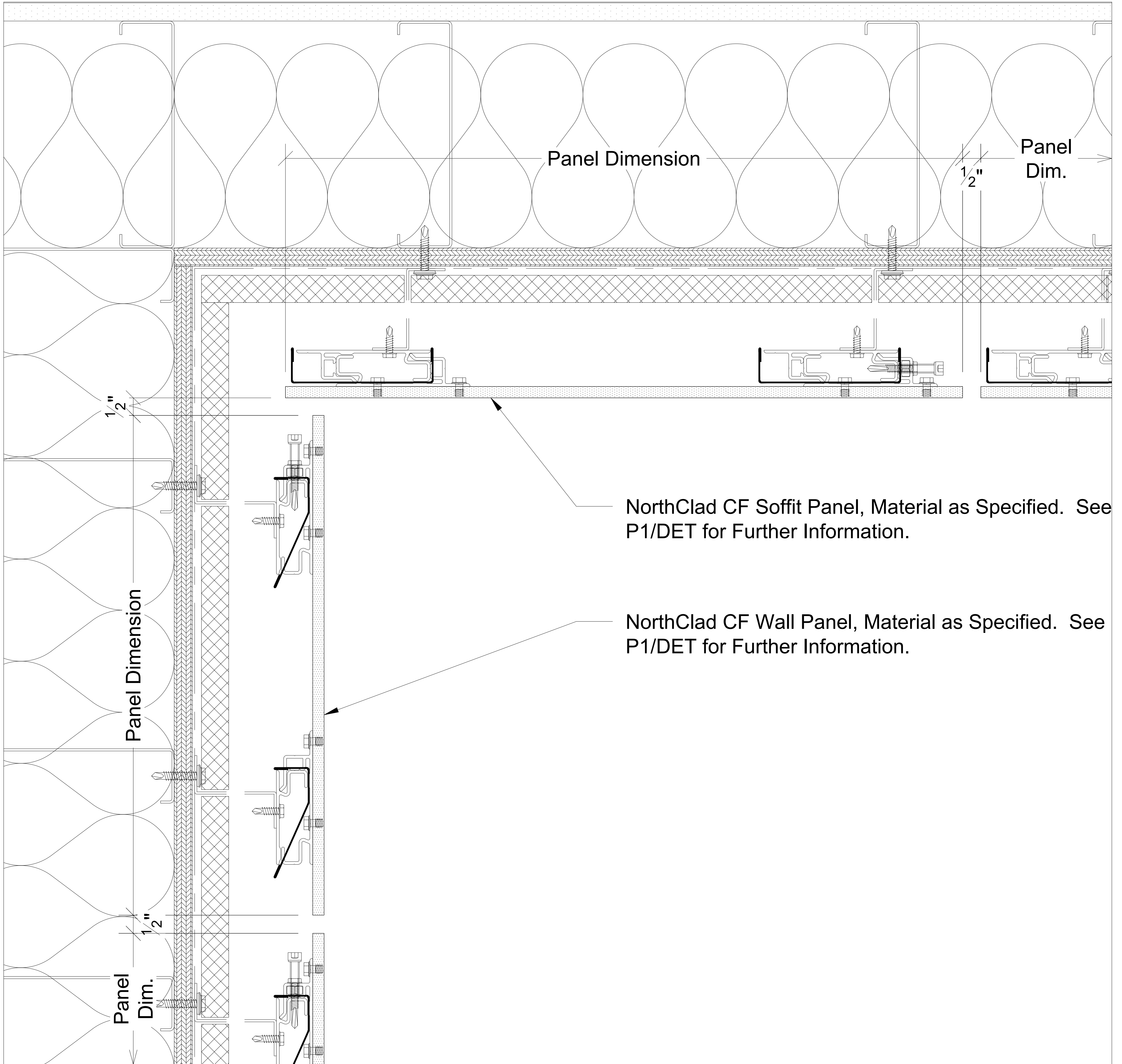
Q1 Section - Soffit at Top of Wall
