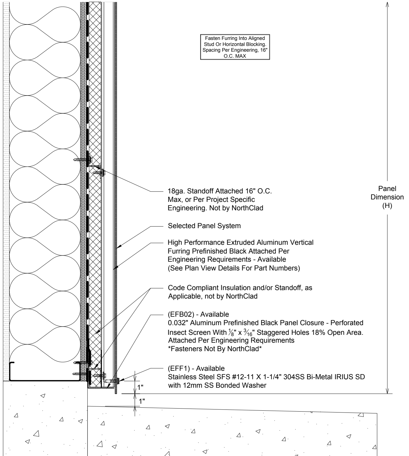
Section - NorthClad EF - Base of Wall System: NorthClad EF System
