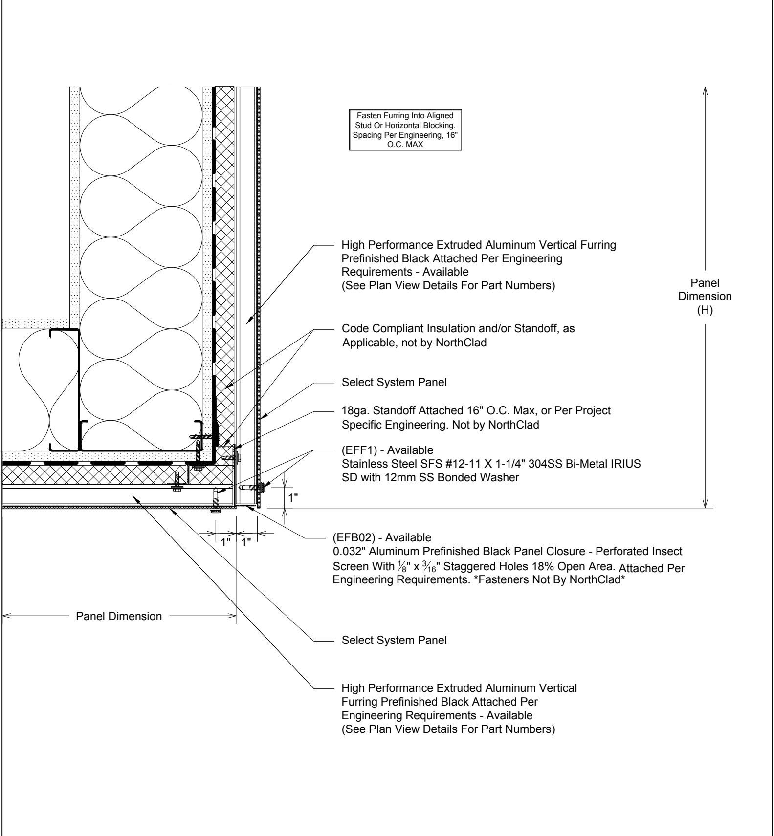
Section - NorthClad EF - Fascia to Soffit System: NorthClad EF System
