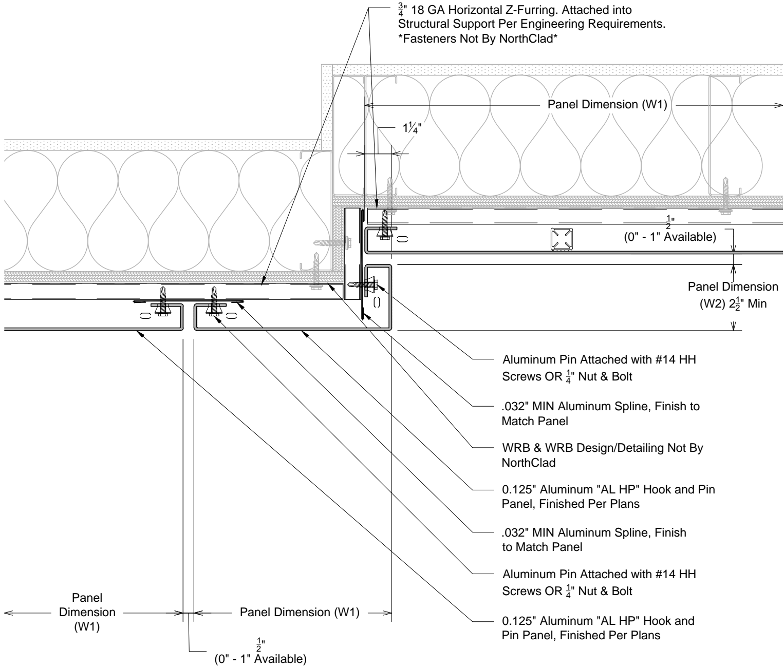
Plan - NorthClad AL HP - Minimum Outside Corner System: NorthClad AL HP System
