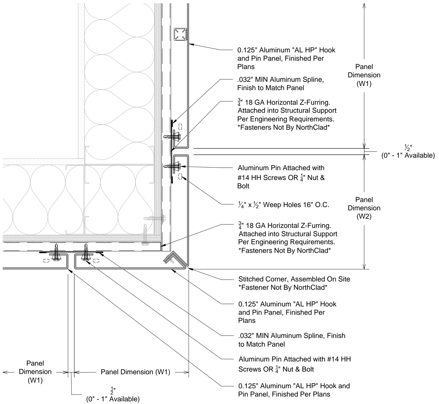
Plan - NorthClad AL HP - Outside Corner Stitched System: NorthClad AL HP System
