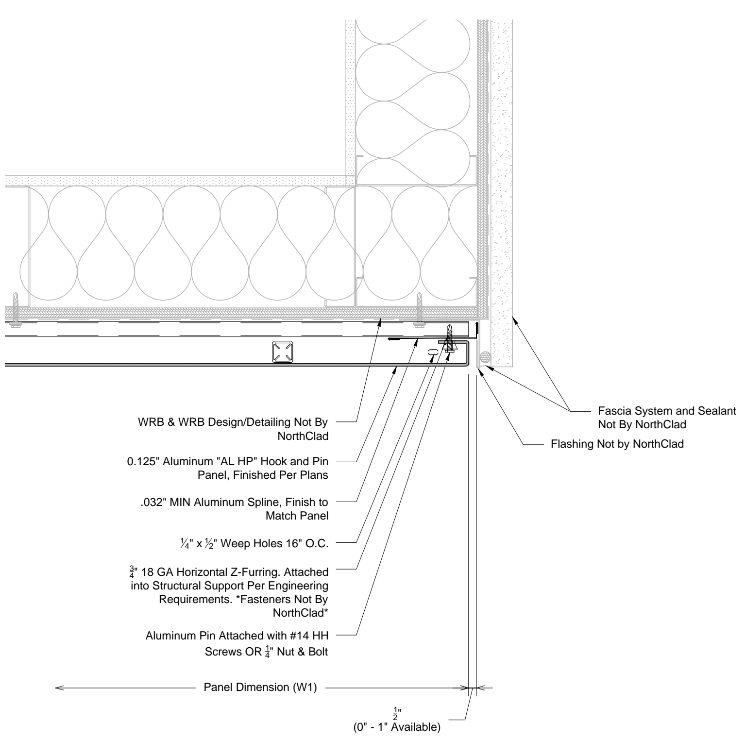
Plan - NorthClad AL HP - Outside Corner to System by Others System: NorthClad AL HP System
