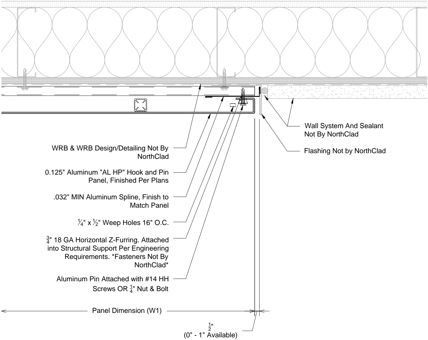
Plan - NorthClad AL HP - Termination to Adjacent Materials System: NorthClad AL HP System
