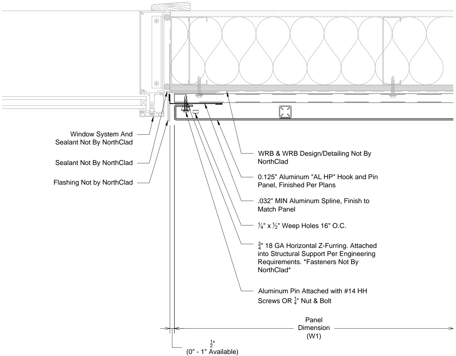
Plan - NorthClad AL HP - Framed Opening Window Jamb System: NorthClad AL HP System
