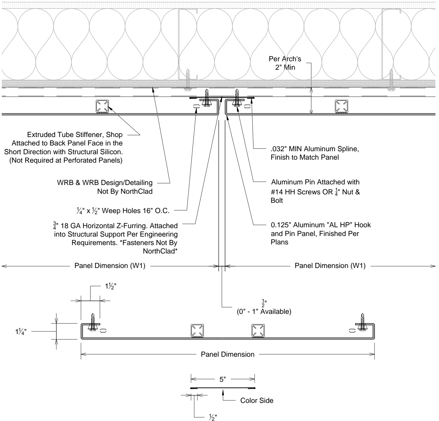
Plan - Vertical Joint System: NorthClad AL HP System
