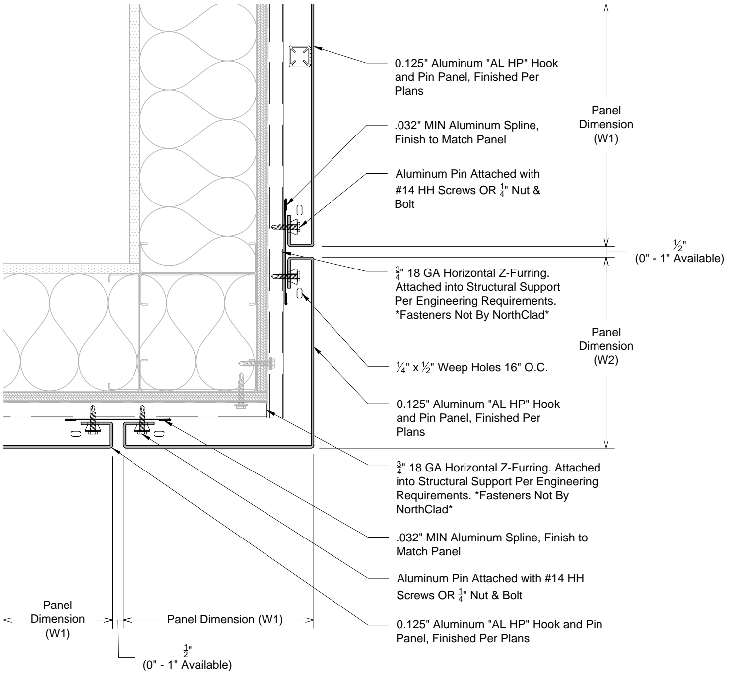
Plan - NorthClad AL HP - Outside Corner System: NorthClad AL HP System
