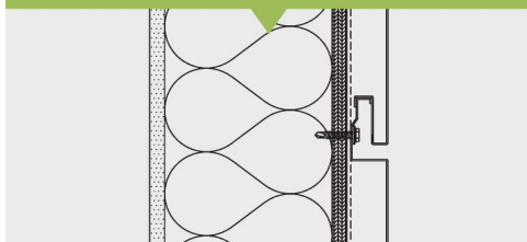
Horizontal Joint
