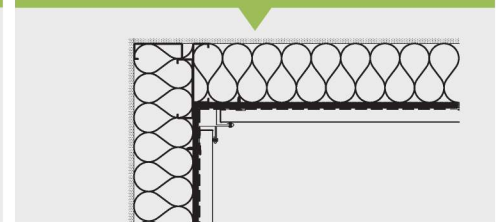
Inside Corner
