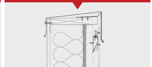
Parapet Coping
