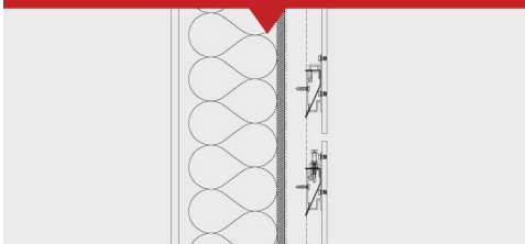
Horizontal Joint
