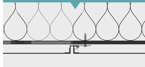
Vertical Joint
