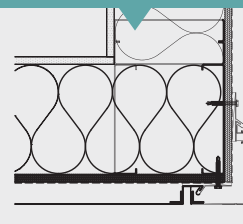
Outside Corner
