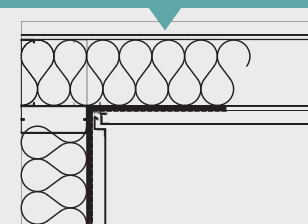
Inside Corner
